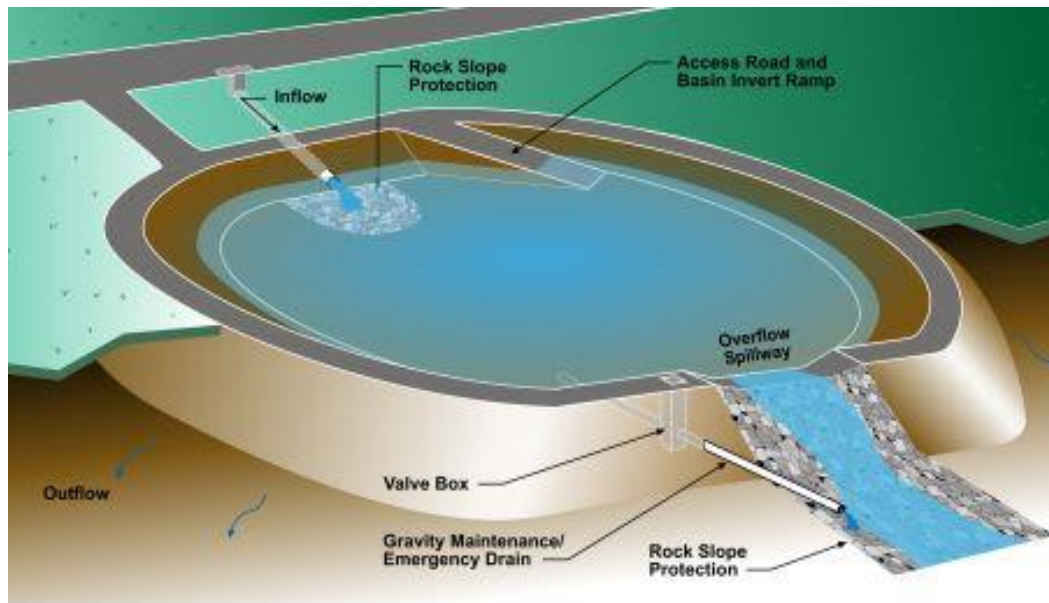
INFILTRATION BASIN
